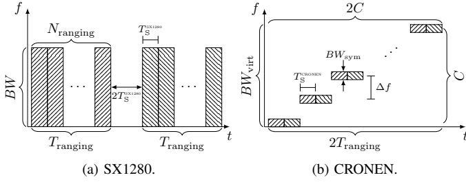
Fig. 5. Spectrum occupation for the two-way ranging protocols.
