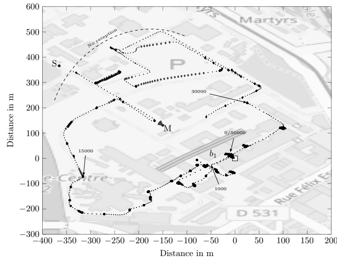
Fig. 9. Ground truth positions for the comparison of LoRa 2.4 GHz SX1280 and CRONEN. Base station (□) at height 26 m and mobile node at height 1.5 m. Mobile node in LoS (●), NLoS (◇) and urban canyon (△) scenario. In bold are stationary position indexes.
