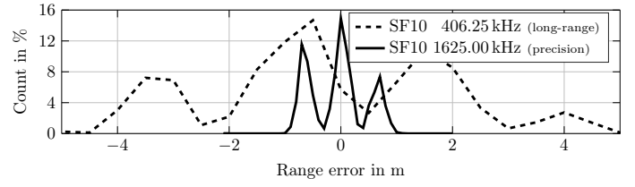
Fig. 6. LoRa 2.4 GHz SX1280 range precision in a cabled AWGN channel for the long-range ( \sigma = 2.1 m) and precision ( \sigma = 0.5 m) configuration.
