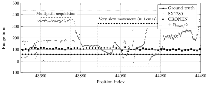
Fig. 11. LoRa 2.4 GHz SX1280 and CRONEN raw range estimates in the urban canyon (zoom).
